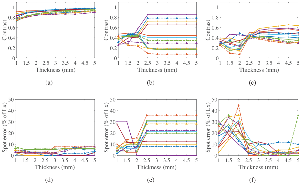
Fig. 7. Contrast and spot error ((a)(d) STIF, (b)(e) TR, and (c)(f) MC) according to the target shape center, respectively at : (—▲— 1(2.,5)) (—▲— 2(3.,5)) (—▲— 3(4.,5)) (—▲— 4(5.,5)) (—▲— 5(2.,6)) (—▲— 6(3.,6)) (—▲— 7(4.,6)) (—▲— 8(5.,6)) (—▲— 9(2.,75)) (—▲— 10(3.,75)) (—▲— 11(4.,75)) (—▲— 12(5.,75)).
