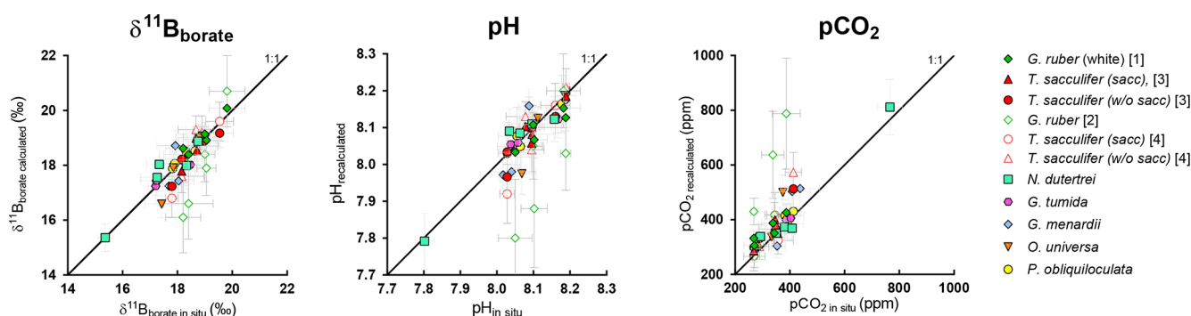
Figure 9. Evaluation of the reconstructed parameters, \delta^{11}\text{B}_{\text{borate}} , pH, and p\text{CO}_2 versus in situ parameters calculated in Fig. 8 (based on \delta^{11}\text{B} and alkalinity). The recalculated parameters are consistent with in situ data, except for G. ruber , and this variability might be explained by the different test sizes within measured size fractions.
