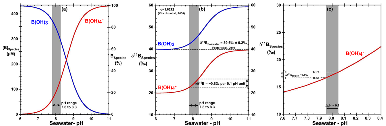
Figure 1. (a) Speciation of B(OH)_3 and B(OH)_4^- as a function of seawater pH (total scale), (b) \delta^{11}B of dissolved inorganic boron species as a function of seawater pH, (c) sensitivity of \delta^{11}B of B(OH)_4^- for a pH ranging from 7.6 to 8.4. T = 25^\circ C , S = 35 , \delta^{11}B = 39.61\text{‰} (Foster et al., 2010), and dissociation constant \alpha = 1.0272 (Klochko et al., 2006).
