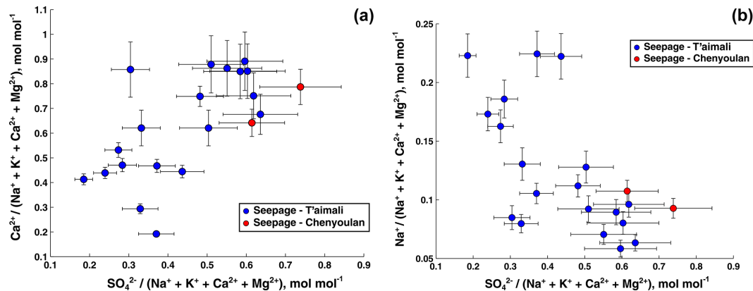
Figure 3. (a) Molar ratio of dissolved calcium to sum of dissolved calcium, magnesium, potassium, and sodium ( \text{Ca}^{2+}/\text{Na}^+ + \text{K}^+ + \text{Ca}^{2+} + \text{Mg}^{2+} ) plotted against ratio of dissolved sulfate to the same dissolved elements ( \text{SO}_4^{2-}/\text{Na}^+ + \text{K}^+ + \text{Ca}^{2+} + \text{Mg}^{2+} ). (b) Molar ratio of dissolved sodium to sum of dissolved calcium, magnesium, potassium and sodium ( \text{Na}^+/\text{Na}^+ + \text{K}^+ + \text{Ca}^{2+} + \text{Mg}^{2+} ) plotted against ratio of dissolved sulfate to the same dissolved elements ( \text{SO}_4^{2-}/\text{Na}^+ + \text{K}^+ + \text{Ca}^{2+} + \text{Mg}^{2+} ). Error bars are the propagated total measurement uncertainty.
