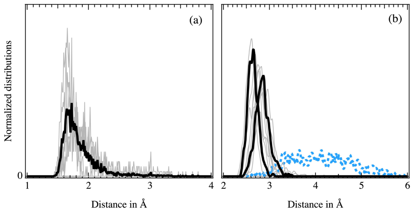
FIG. 6. Geometrical details of the ionic interactions between the M^{\text{Pro}} catalytic dyad and the inhibitor ketoamide moiety. (a) Normalized distributions of the distance R_1 between the hydrogen HE2 (PDB labeling) of His 41 and the ketoamide oxygen O 1 [see Fig. 2(a) for definition]. (b) Normalized distributions of the distances R_2 between the thiolate sulfur of Cys 41 and the two ketoamide sp^2 carbons. Light gray and bold black lines: distributions for individual inhibitor and averaged over all inhibitors, respectively, with the exception of 11f whose specific R_2 distributions are shown in blue dashed lines.
