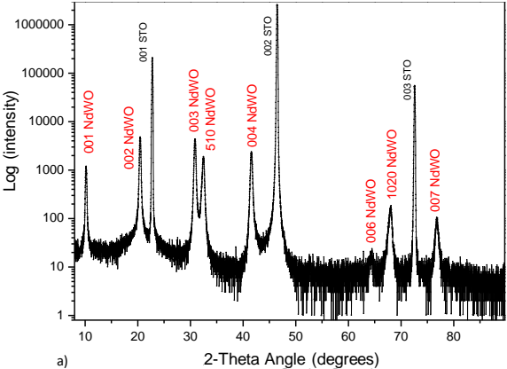
Figure 2. X-ray diffractograms on \text{Nd}_2\text{WO}_6 thin films. (a) 2\theta - \omega X-ray diffractogram of \text{Nd}_2\text{WO}_6 thin film grown at T=900^\circ\text{C} and \text{PO}_2 = 10^{-1} mbar. (b) Normalized rocking curves on 002 \text{NdWO} thin film and on 001 STO substrate (FWHM are indicated in inset).
