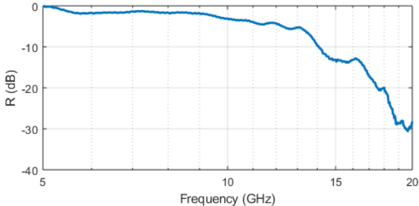
Figure 2. Modulator response for a -15V bias voltage (normalized).
