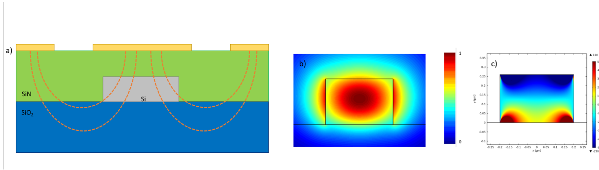
Figure 1. a) Schematic view of the cross-section of one MZM arm. Orange dotted lines represent the electric field lines. b) Distribution of the TE mode in the cross section (normalized). c) \chi^{(2)} distribution (pm/V) in the cross section of the waveguide.
