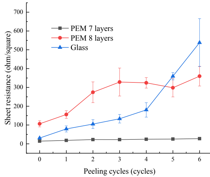
Fig. 7. Plot of the sheet resistance of the AgNW coated on glass, PEM 7 and 8 layers as a function of the number of peeling cycle
