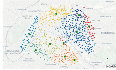
(b) Results of our modified Robust EM on week 12.
