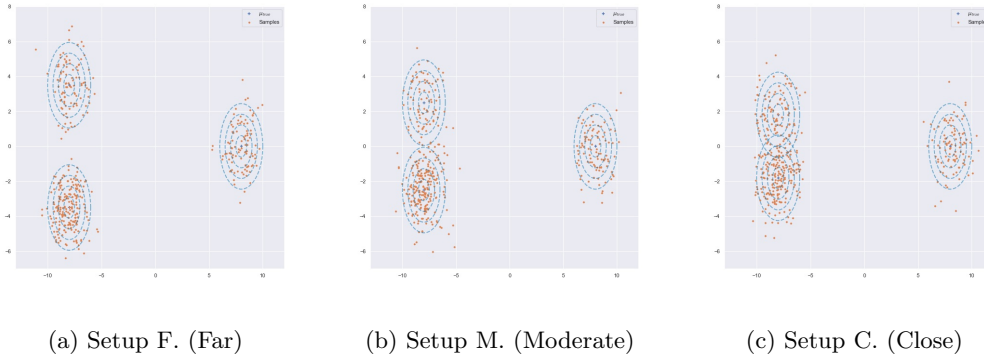
Figure 4: Gaussian mixture distributions for Setups F., M. and C. involved in Cases presented in Table 2 with an example of sampled data sets. Blue crosses correspond to \mu_k and ellipsis to covariance matrices \Sigma_k . Orange points are samples.
