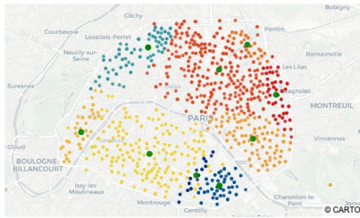
(c) Results of the original Robust EM on week 13. We observe here overlapping clusters.
