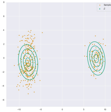
Figure 5: An estimated GMM with \hat{K} = 2 \neq K_{true} = 3 for a Setup C. distribution. The centers and covariances are represented in green. Orange points are samples.
