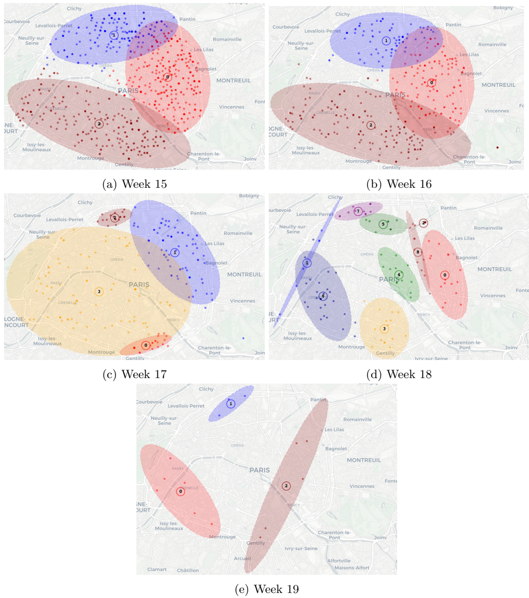
Figure 8: Estimated Gaussian Mixture Models on COVID-19 dataset per week (weeks 15 to 19).
