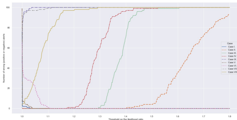
Figure 2: For each Case is presented the number of false alerts (positive or negative) depending on estimated likelihood ratios given by (5), over S = 100 runs according to the considered threshold \tau . The filled black vertical line is the final selected threshold. Datasets are of size n = 400 .
