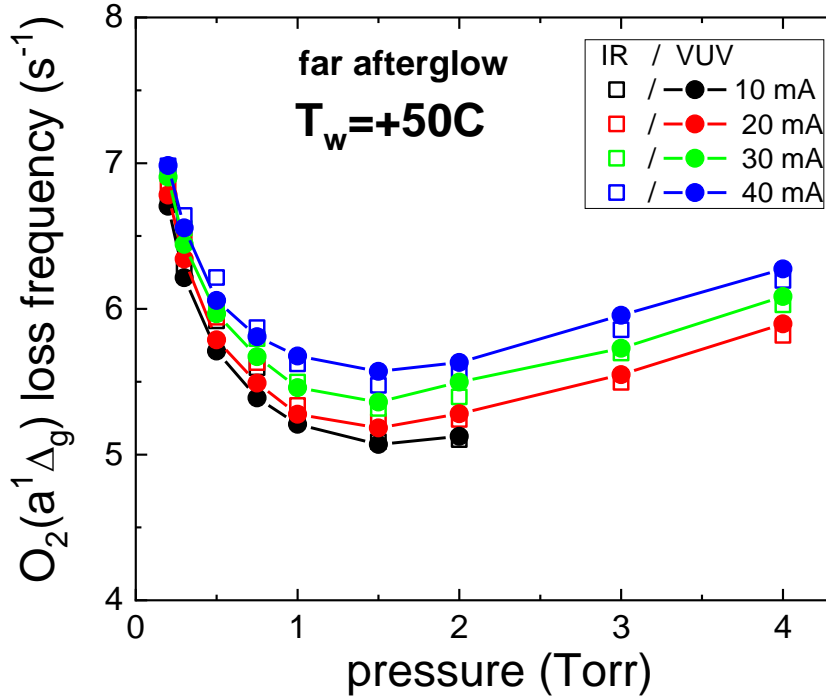
Figure 5. The O_2(a^1\Delta_g) loss frequency in the late afterglow obtained from the IR emission decay as function of pressure for different currents. The O_2(a^1\Delta_g) loss frequency determined from the rate of recovery of the O_2(X^3\Sigma_g^-) density in the later afterglow (measured by VUV absorption) is also shown (see below).
