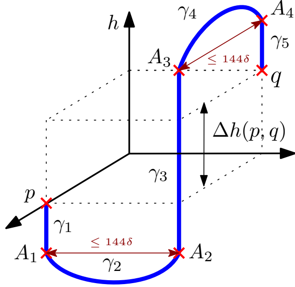
Figure 12: Construction of the path \gamma when h(p) \leq h(q) for Lemma 4.10.
