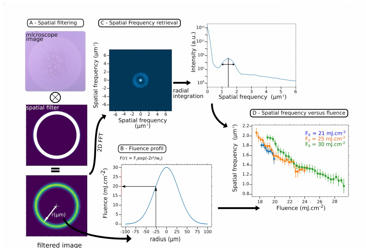
Figure 2. Analysis of the wrinkles' spatial frequency as a function of the impinging fluence determined by selecting different rings of various radius in the wrinkles' circular area.
