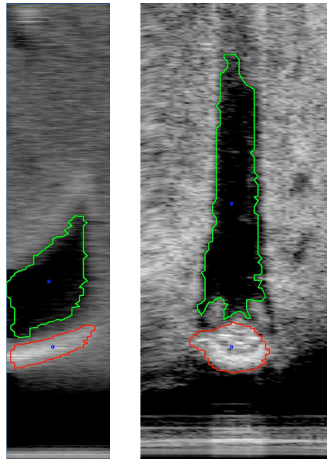
Figure 5: Classification results on a Cylinder and a Manta mine.
