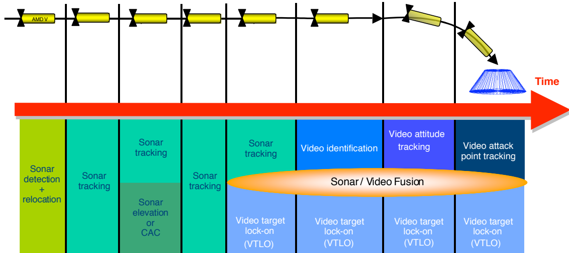
Figure 1: operational phases for AMDV. Sonar modules are in green and video modules in blue.
