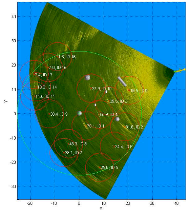
Figure 3: Sample detection phase sonar data with results superimposed on it.
