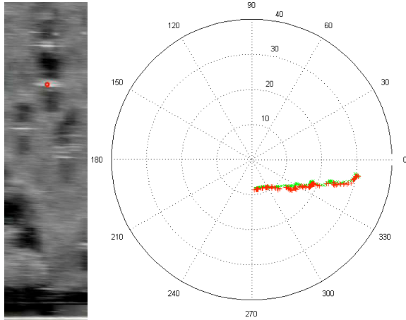
Figure 4: Sonar approach results
