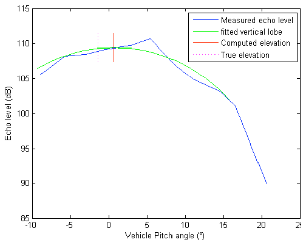
Figure 6: One elevation estimation result done at 20 m from the mine.
