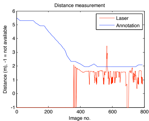
Figure 8: raw laser range measures vs. manual annotation for a Manta mine. Value -1 means "no measure".
