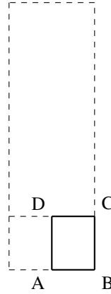
Figure 28: Simplified modeling of the problem. Symmetry boundary condition is applied on AD , contact and heat flux on AB , free tractions on BC and imposed displacement on DC .
