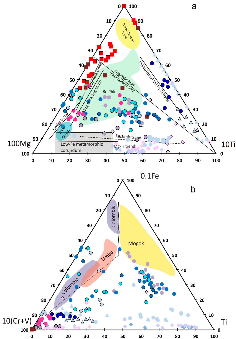
Figure 11. Greek corundum LA-ICP-MS analyses plotted on a (a) Mg \times 100 - Fe - Ti \times 10 discrimination diagram. Also shown are the metamorphic Fe–Mg and Fe–Ti trends of Mogok and low-Fe sapphires of Pailin, Ilakaka and Ratnapura Balangoda, the Umba and Kashmir trends of metasomatic blue sapphires, and the Bo Phloi scattering of atypical blue sapphires (modified after Peucat et al. [16]); (b) Fe \times 0.1 - (Cr + V) \times 10 - Ti diagram for Colombia, Mogok and Umba blue sapphires along with the plots from the Greek corundums, modified after Peucat et al. [16]. Symbols as in Figure 9.
