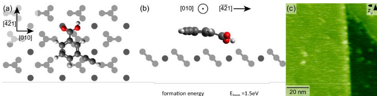
Figure 2. Optimized geometry of an isolated 3-EBA molecule on the calcite (10.4) surface in (a) top view and (b) side view. (c) AFM topography image of an as-deposited calcite (10.4) sample. Two step edges are seen in the image. The terraces are covered by streaky features, indicating mobile species on the surface at room temperature.
