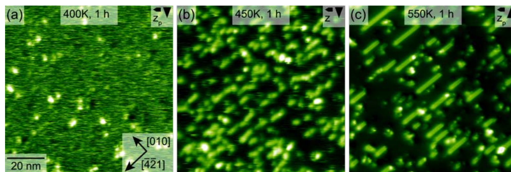
Figure 3. Examples from a heating series of a molecule-covered sample. Each annealing step lasted for 1 hour. (a) Heating to 400 K led to the formation of some bright dots, while (b) heating to 450 K resulted in a reduction of the streaky features and the appearance of stripe-like structures, oriented in the [-4-21] direction. Further heating to (c) 550 K yielded in longer stripes and the disappearance of the streaky features.
