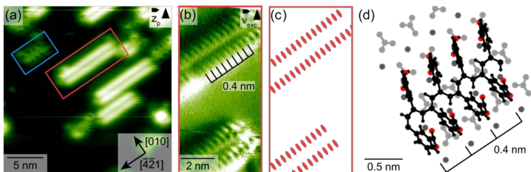
Figure 4. Molecular structure obtained upon heating the sample for 1 h to 550 K. (a) Two different kind of stripes can be seen along the [-4-21] direction, marked by red and blue boxes, respectively. (b) The stripe marked by the red box in (a) is shown in a frequency shift image, revealing the periodicity of 0.4 nm. (c) Sketch illustrating the inner structure of the stripes. (d) Acetylene polymer structure as obtained from DFT, including the calcite (10.4) surface to illustrate the excellent match in size and pattern.
