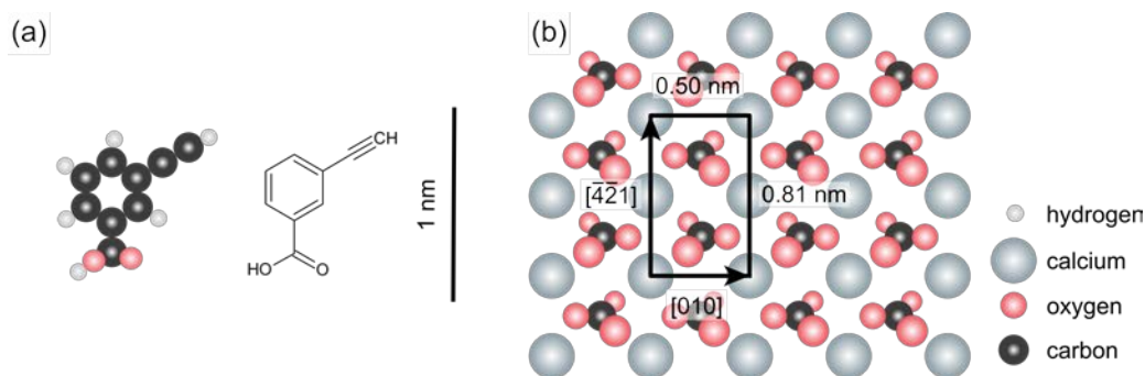
Figure 1. Model of (a) the 3-ethynylbenzoic acid (3-EBA) molecule and (b) the calcite (10.4) surface. The scale bar applies to both models. The calcite (10.4) surface has a rectangular unit cell with dimensions of (0.50 \times 0.81) \text{ nm}^2 , consisting of two carbonate ions and two calcium ions.
