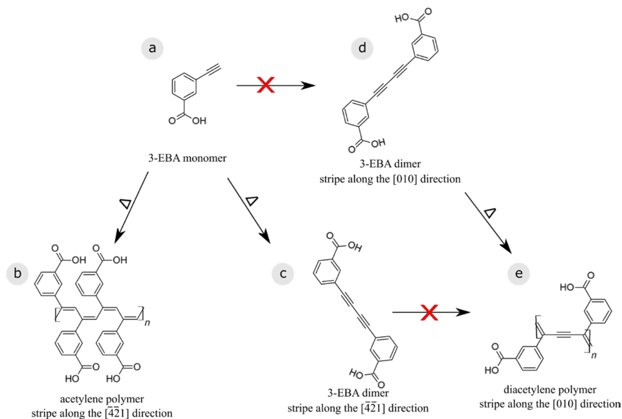
Figure 6. Overview of the reaction pathways of the 3-EBA monomer (a) on calcite (10.4). Upon annealing, acetylene polymerization can be induced (b). The monomer can also form homo-coupled dimers. These dimers align side-by-side and form rows along the [\bar{4}-21] direction (c). Interestingly, in this arrangement, the dimers do not react further. When directly depositing the dimers, rows arranged in the [010] direction form (d). Only in this arrangement, the dimers undergo diacetylene polymerization (e).
