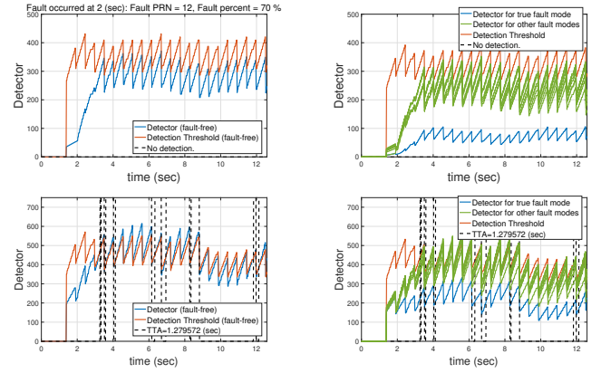
Fig. 8. Fault detector and threshold values of the full-set filter (left) and the sub-set filters (right) without (top) and with vision (bottom)
