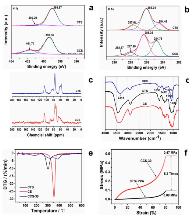
Figure 2. a) High-resolution N 1s spectra; the N 1s (399.36)/N 1s (401.71) of the chitosan/cellulose sponge (CCS) is weaker than that of chitosan (CTS), indicating that some amino groups reacted with glutaraldehyde. b) C 1s of spectra from XPS analysis; compared to chitosan the broad peaks of C1s of chitosan/cellulose sponge at 287.9 eV correspond to imine bonds C=N. c) 13 C solid-state NMR spectra of chitosan/cellulose sponge and chitosan are very similar, new peaks at 100.1 ppm and 129.5 ppm can be attributed to conjugated ethylene bonds, and imine bonds at 179 ppm. d) Fourier transform infrared spectroscopy show that the peak at 1638 cm -1 is due to C=O stretching of amide I; the C=N bond band formed by crosslinking chitosan and glutaraldehyde also appear in this region, thus proving the Schiff base reaction. e) Derivative thermogravimetric (DTG) curves: the mass loss differences of chitosan, cellulose (CE), and chitosan/cellulose sponge indicate that the crosslinking was successful. f) Compressive stress-strain curves show that under 80% strain the cross-linking of chitosan improved the mechanical strength of the material and the compressive strength. PVA: polyvinyl alcohol. [21] Copyright © 2019 Elsevier B.V.
