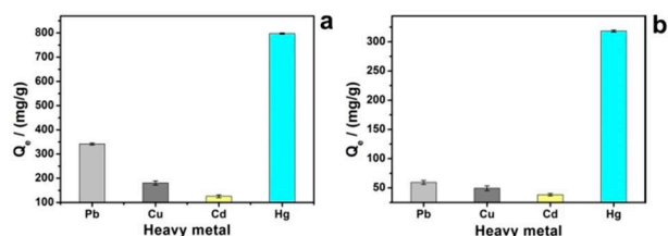
Figure 10. Selective adsorption by hyperbranched polyethylenimine-functionalized carboxymethyl chitosan composite. Sample dosage 20 mg/20 mL, temperature 30 °C, pH 5.5, adsorption time 360 min. a) Single component solution; b) Mixed component solution. [20] Copyright © 2019 Elsevier B.V.
