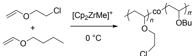
Scheme 38. Cationic copolymerization of BVE and CEVE.
