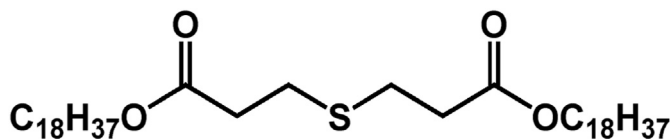
Fig. 2. Chemical structure of DSTDP.
