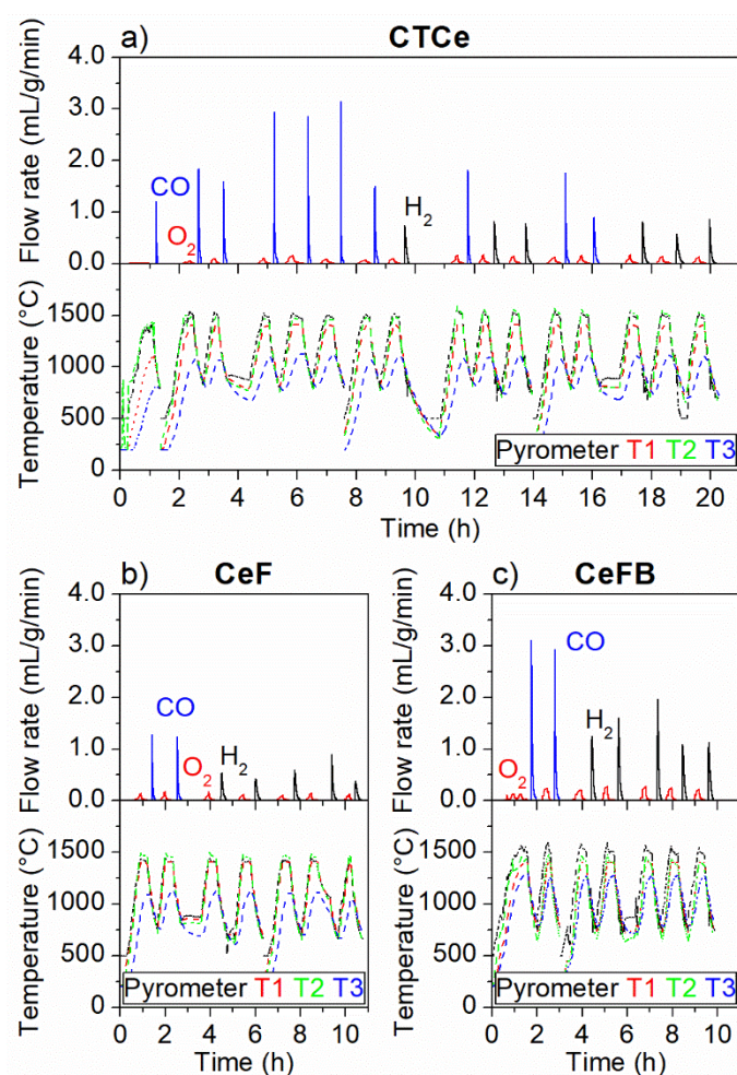
Figure 3: O 2 and fuel production rates during the performed cycles along with the temperature profiles for a) CTCe (16 cycles), b) CeF (7 cycles) and c) CeFB (7 cycles). T1, T2 and T3 are the temperatures of the sample interior, sample surface and the base of the reactor.
