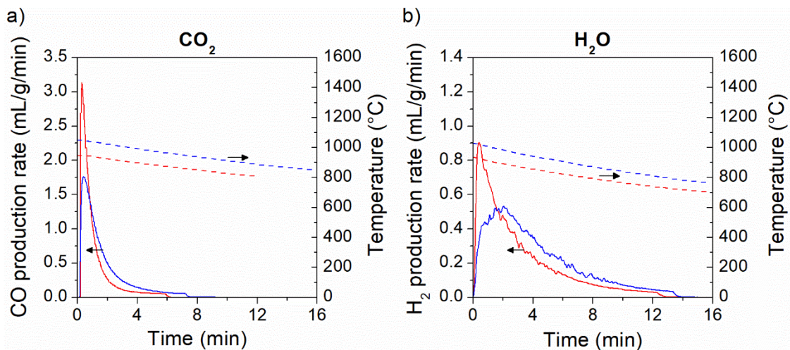
Figure 6: a) \text{CO} production rate from CTCe (solid lines) along with T_1 temperature (dashed lines) for 949^\circ\text{C} (cycle #6) and 1054^\circ\text{C} (cycle #12) starting oxidation temperature and b) \text{H}_2 production rate from CeF (solid lines) along with T_1 temperature (dashed lines) for 1039^\circ\text{C} (cycle #3) and 940^\circ\text{C} (cycle #6) starting oxidation temperature
