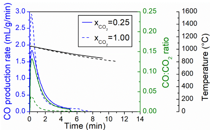
Figure 9: CO production rates from CTCe (blue lines) along with the associated CO:CO 2 ratio (green lines) and T1 temperature (black lines) for a CO 2 molar fraction ( x_{CO_2} ) of 0.25 (solid lines, cycle #2) and 1.00 (dashed lines, cycle #4)
