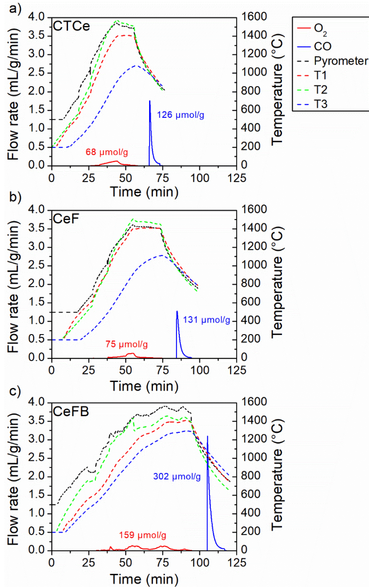
Figure 4: Thermochemical cycles at atmospheric pressure, T_{red}=1400^{\circ}\text{C} and T_{ox}=1050^{\circ}\text{C}-850^{\circ}\text{C} with 50mol% \text{CO}_2 during the oxidation step for a) CTCe (cycle #12), b) CeF (cycle #1), and c) CeFB (cycle #1)
