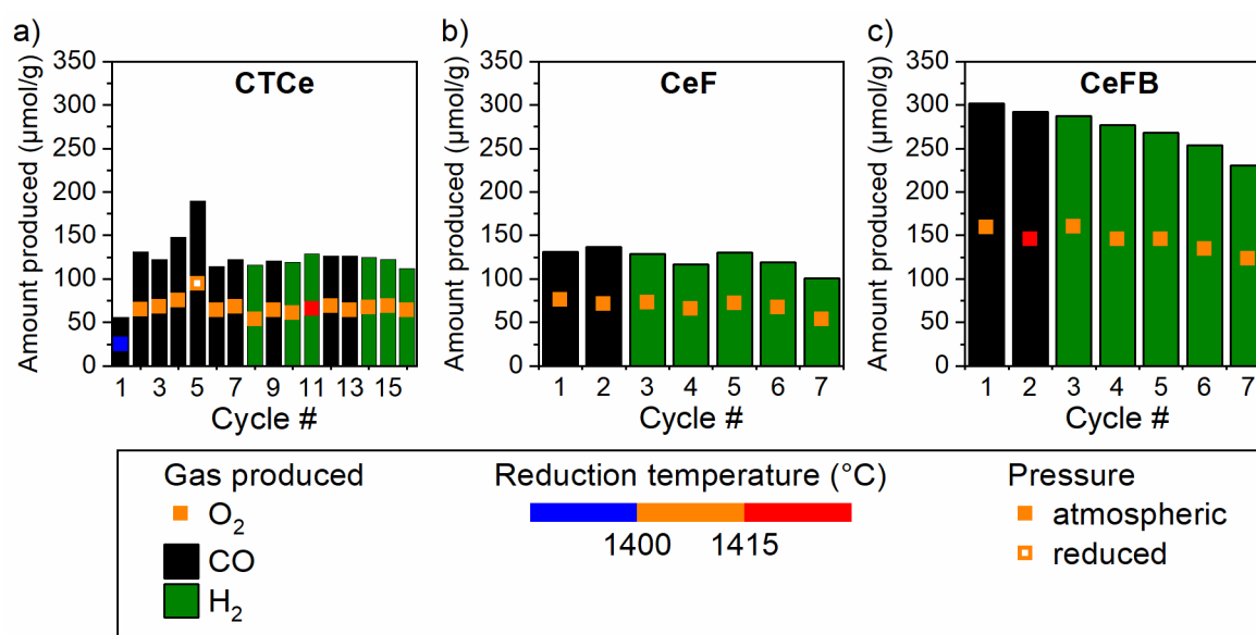
Figure 5: O 2 and fuel production yields over cycles for a) CTCe, b) CeF and c) CeFB; squares represent the O 2 production amount and bars refer to the fuel production. The reduction temperature is indicated by the color of the square.
