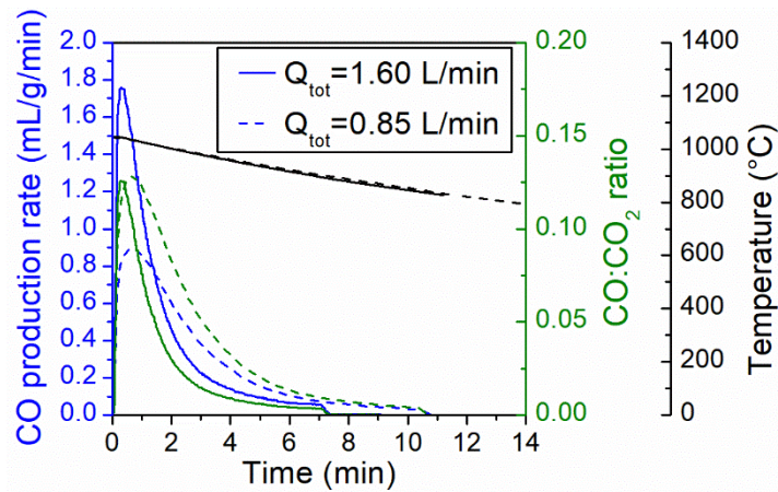
Figure 7: CO production rate from CTcE (blue lines) along with \text{CO}:\text{CO}_2 ratio (green lines) and T_1 temperature (black lines) for different total flow rates during oxidation step: 1.60 L/min (solid lines, CTcE cycle #12) and 0.85 L/min (dashed lines, CTcE cycle #13) with x_{\text{CO}_2} = 0.25 .
