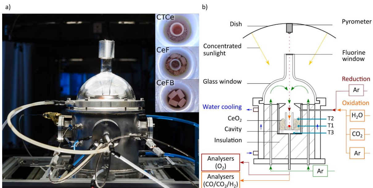
Figure 1: a) Photograph of the solar reactor, image inserts on the right show CTce, CeF and CeFB (from top to bottom) inside the alumina cavity and b) schematic illustration of the solar reactor, red arrows represent the gas flow during the reduction step, orange arrows the gas flow during the oxidation step, green arrows the Ar flow injected during both steps to protect the glass window and sweep the cavity, and blue arrows the water-cooling.
