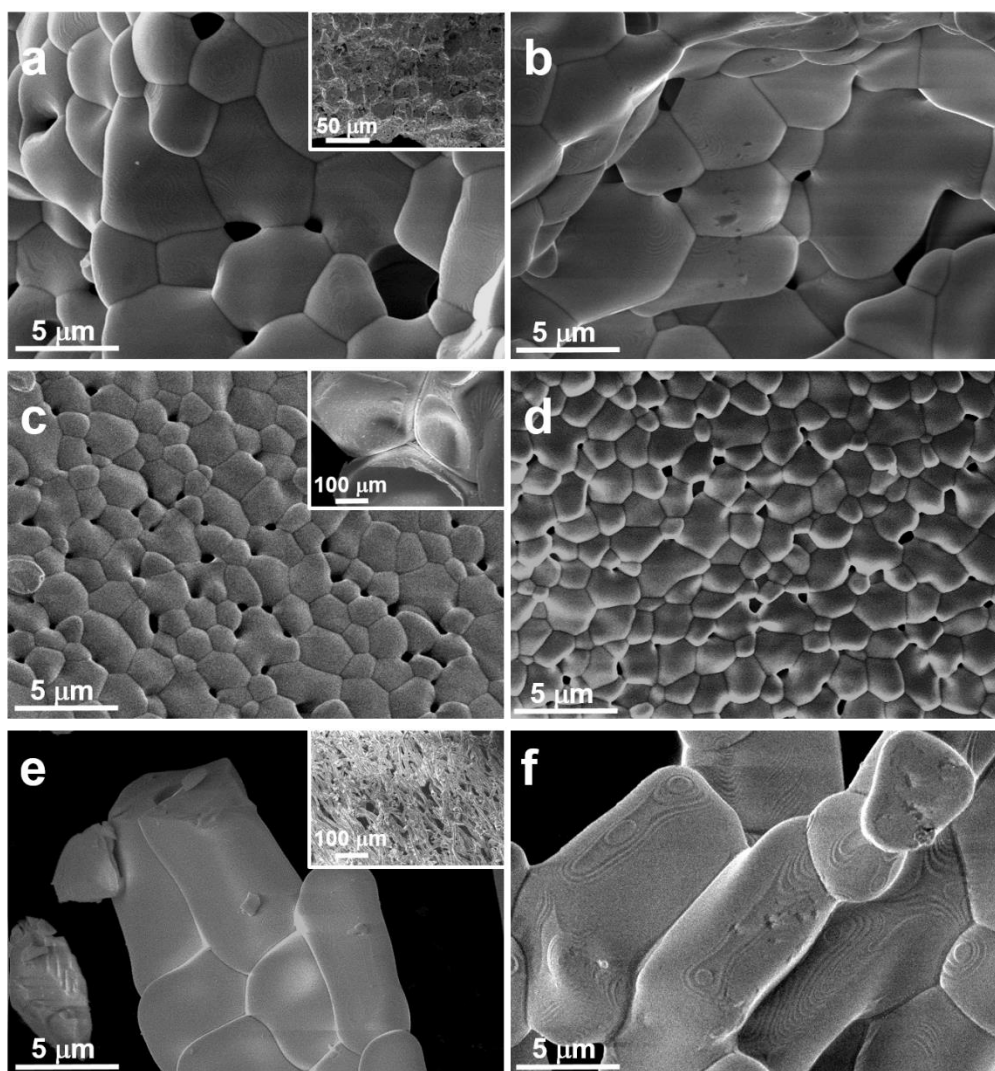
Figure 11: Comparison of representative microscopy images of CTCe, CeF and CeFB prior (a, c, e) and after (b, d, f) thermal cycling. Inserts are images taken at lower magnification.
