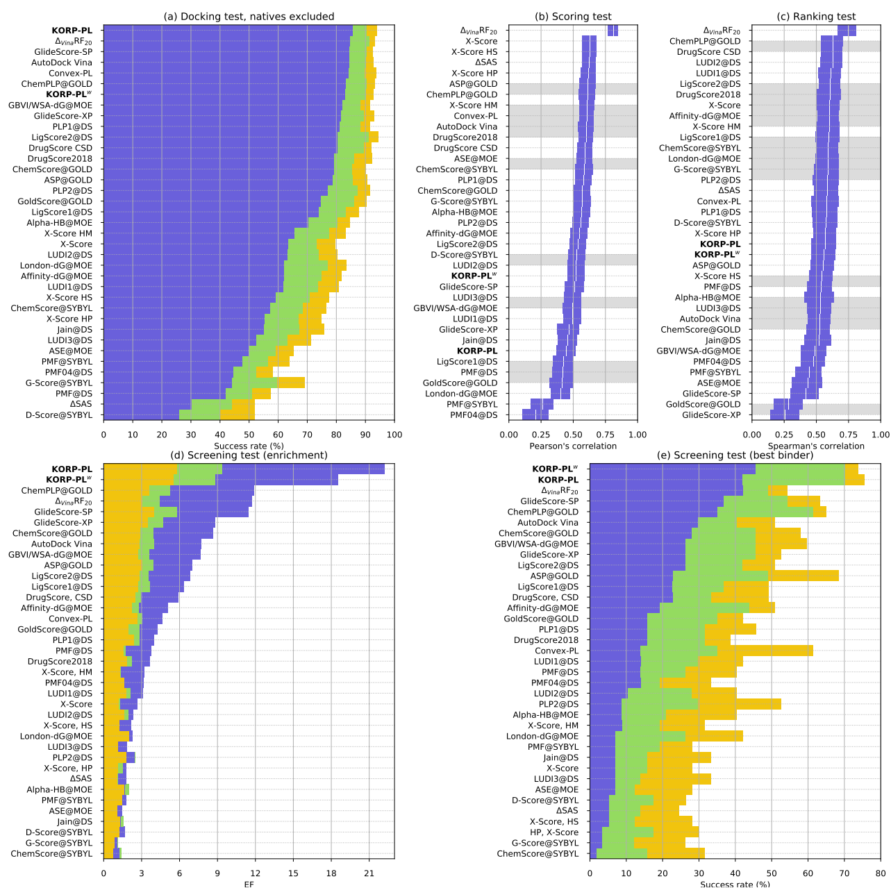
Fig. 2. CASF-2016 benchmark results. (a) The success rate of finding a near-native pose within 2 \text{ \AA} RMSD in Top 1 (blue), Top 2 (green), and Top 3 (yellow) predictions. Native poses are excluded. (b) Pearson's correlation with confidential values between predicted scores and experimental \log K_a . Scoring functions sharing the same gray bar are not distinguishable at \alpha = 0.1 in the post-hoc Friedman test (Su et al., 2018). (c) Spearman's rank correlation with confidential values among the 57 clusters. (d) Enrichment factors computed considering 1% (blue), 5% (green), and 10% (yellow) of the top-ranked compounds. (e) The success rate of identifying the highest-affinity binder among the 1% (blue), 5% (green), or 10% (yellow) top-ranked ligands. All results except Korp-PL and Convex-PL were taken from the supplementary information of the CASF-2016 benchmark paper (Su et al., 2018). The results of Korp-PL, Korp-PL w , and Convex-PL are available in Tables S3-S5 of SI.
