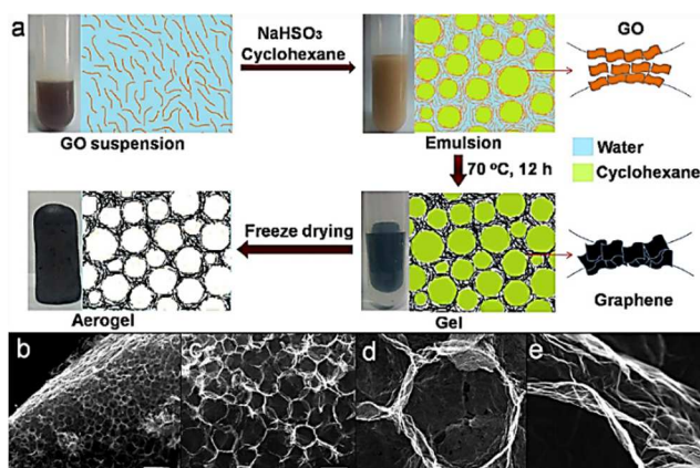
Figure 10 Synthesis process of GA from the assembly of GO at oil-water interface and the subsequent chemical reduction, complementary with the SEM images. (a) GO concentration of 2 \text{mg mL}^{-1} , (b) emulsion of GO, \text{NaHSO}_3 and cyclohexane, (c) graphene hydrogel with hexagonal pore connecting the boundary with six other identical pores, providing a strong linking bridge, (d) view of the GA. Reproduced with permission from Ref. 134 , Copyright Nature Publishing Group 2016.
