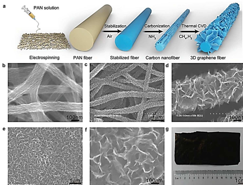
Figure 7 Preparation process and structure of the 3D graphene fibers. a) A schematic illustration of the preparation process. b) A SEM image of the carbon fibers carbonized in \text{NH}_3 . c,d) SEM images of the 3D graphene fibers grown for 4 h at \text{CH}_4 concentration of 11.1% and 1100 \text{ }^\circ\text{C} . e,f) SEM images of the 3D graphene fibers grown for 10 h at \text{CH}_4 concentration of 11.1% and 1100 \text{ }^\circ\text{C} . g) An optical image of the 3D graphene fibers membrane. Reproduced with permission from Ref. 96 , Copyright Wiley-VCH 2018.
