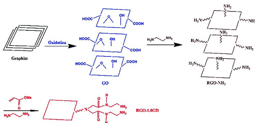
Figure 11 Possible mechanism of PAMAM grafting onto GO nanosheets to form 3D porous graphene network. Reproduced with permission from Ref. 149 , Copyright The Royal Society of Chemistry 2016.
