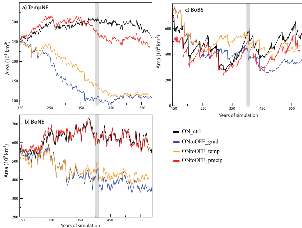
Fig. 13. Area of Western Europe (lat = 32/60^\circ , lon = -15/20^\circ ) occupied by (a) Temperate needleleaf evergreen; (b) Boreal needleleaf evergreen; (c) Boreal broadleaf summergreen trees in ON_ctrl (black), ONtoOFF_grad (blue), ONtoOFF_precip (red) and ONtoOFF_temp (orange). The vertical grey bars indicate when the AMOC is fully collapsed in ONtoOFF_grad.
