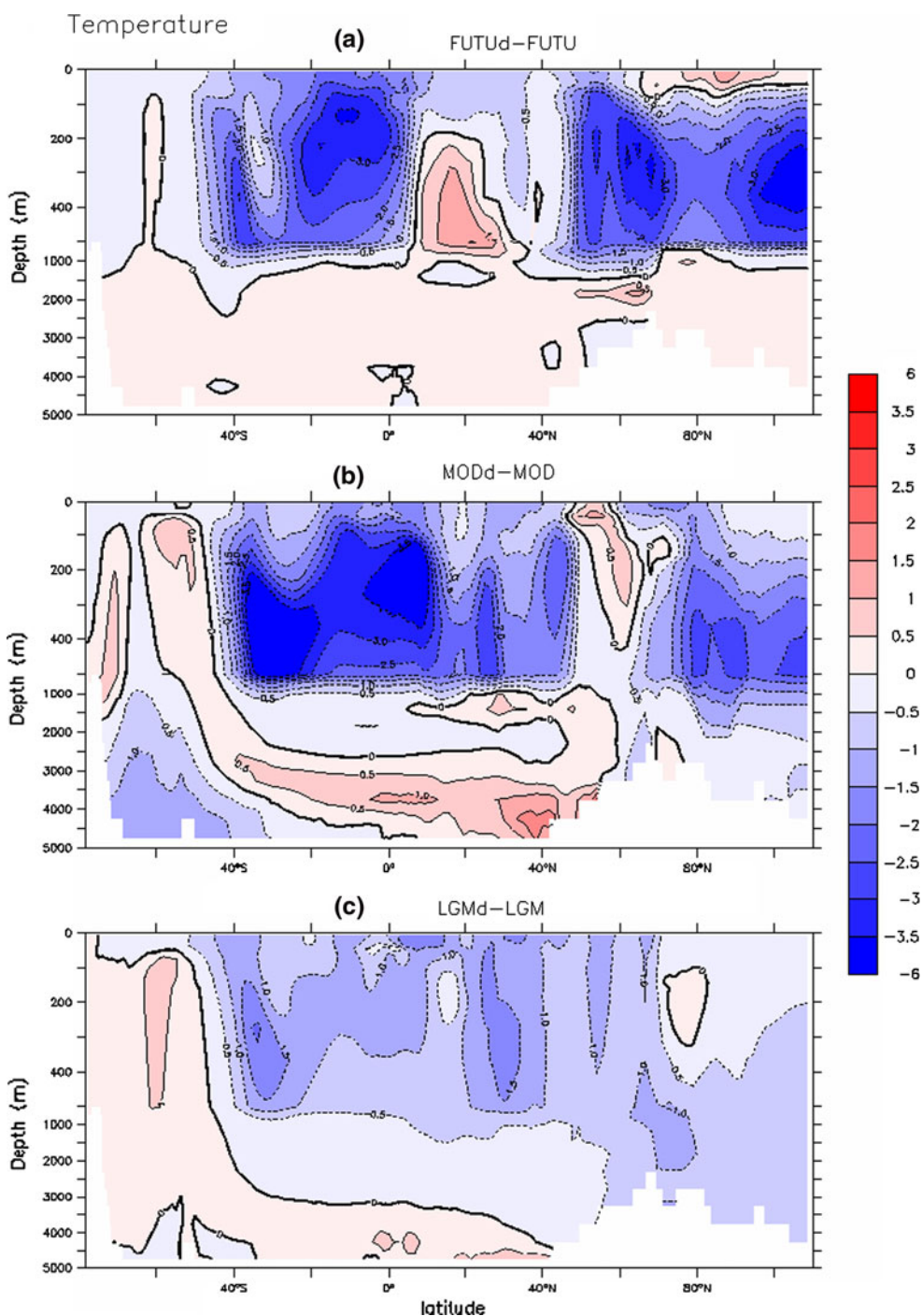
Fig. 11 Atlantic latitude-depth sections temperature a FUTd-FUT b MODd-MOD and c LGMRd-LGMR
