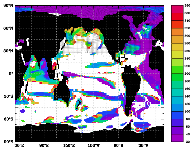
Fig. 9. FFW–GLA time response (in years) of EXP (export production): defined as the time after which half of the final signal (averaged on the simulated years 350–399) in EXP has been reached. We only considered regions where the final anomaly of EXP was more than 1 \text{ gC m}^{-2} \text{ yr}^{-1} in absolute value: the white areas in the ocean do not have such an important anomaly in the end.
