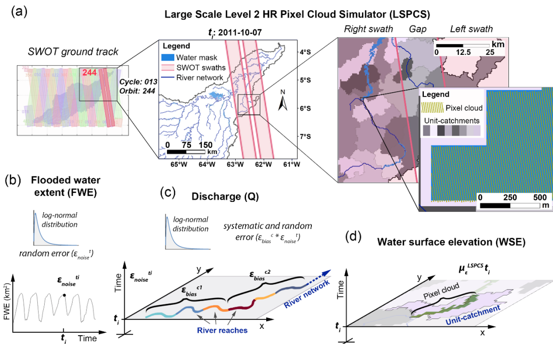
Figure 5. Schematic framework of the (a) Large Scale Level 2 HR Pixel Cloud Simulator (LSPCS) for specific day t_i and the adopted perturbation to generate the SWOT-like observations for (b) Flooded Water Extent (FWE), (c) Discharge (Q), and (d) Water Surface Elevation (WSE).
