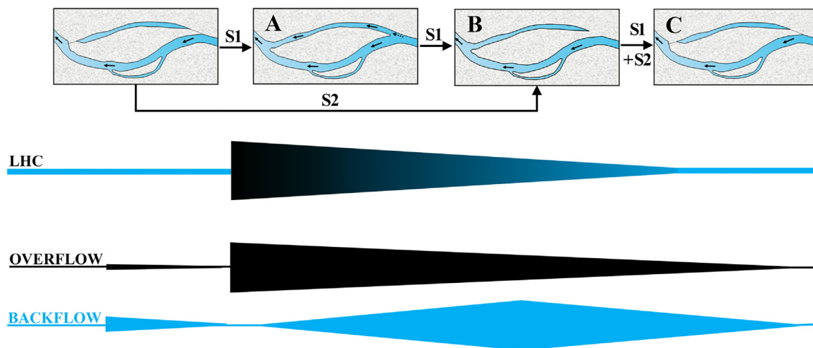
Fig. 1. Two scenarios S1 and S2 of floodplain channel succession: A – Upstream overflow dominated channel (fully connected, essentially lotic; eutotamion); B – Backflow dominated channel (semi-connected, semi-lotic; parapotamion); C – Progressive disconnection of the floodplain channel (isolated, predominantly lentic; plesiopotamion). The color gradient refers to the relative importance of the two flow processes: overflow (black) and backflow (blue) connections in the lateral hydrological connectivity (LHC). (For interpretation of the references to color in this figure legend, the reader is referred to the web version of this article.)
