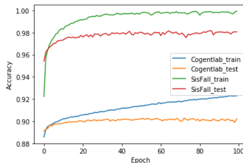
Figure 2: Model accuracy evolution through 100 epochs
