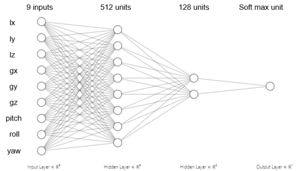
Figure 1: ANN architecture
