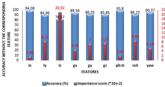
Figure 4: Features importance for SisFall
