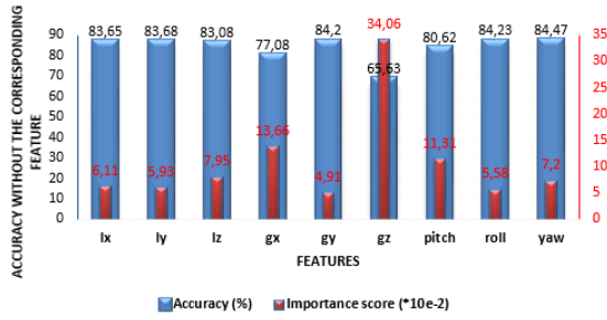
Figure 3: Features importance for Cogentlab
