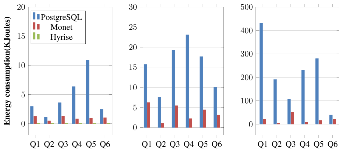
(a) On TPC-H when SF=5 GB (b) On TPC-H when SF=30 GB (c) On TPC-H when SF=100 GB
