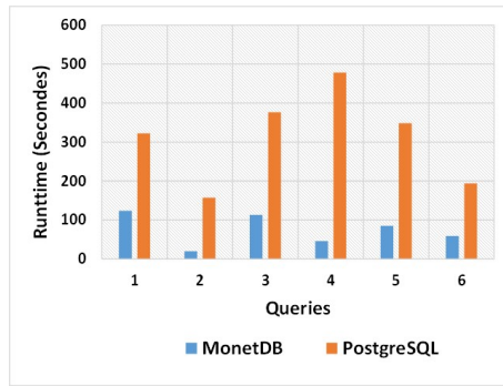
(c) On TPCH SF30
