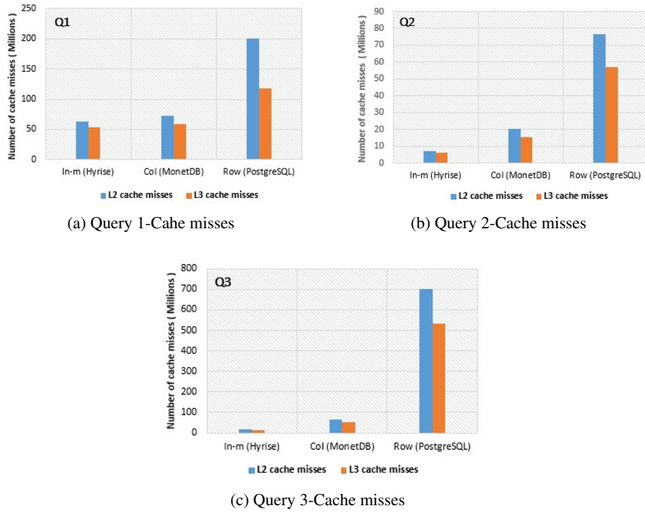
Figure 9 – LLC and L2 cache misses for Q_1, Q_2, Q_3 queries from TPC-H benchmark.
