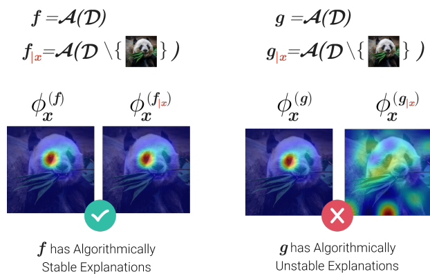
Figure 1. The explanations of a predictor f can be trusted when they are algorithmically stable. It means that, on average, for any image \mathcal{x} removed for the training set \mathcal{D} , another predictor f_{|\mathcal{x}} trained with the same algorithm \mathcal{A} produces a similar explanation for the same input image. This stability ensures that the explanations of correctly classified images of the same class will point out similar evidence of the class. For instance, the explanations for the class panda will all point out the black area around their eyes.
