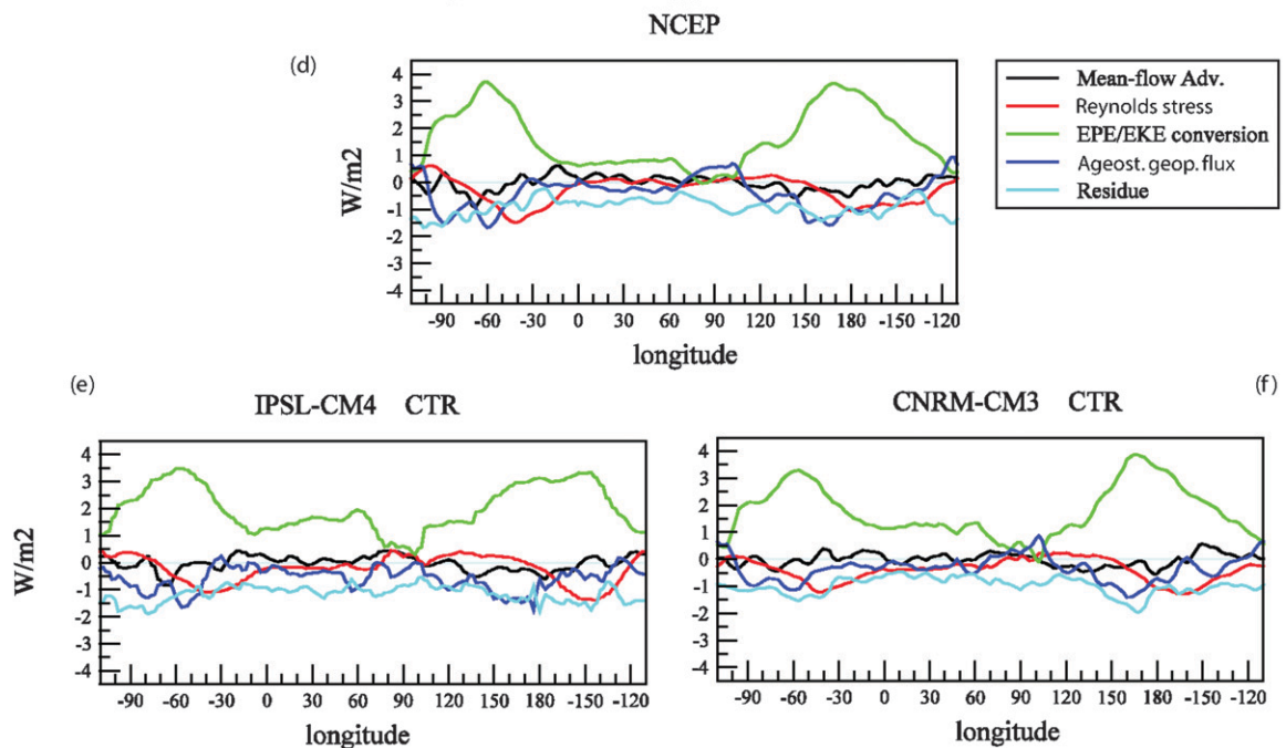
FIG. 4. DJF eddy (band passed) potential energy conversion terms [cf. Eqs. (1) and (3)] and DJF eddy kinetic energy conversion terms [cf. Eq. (2)] integrated from 925 to 200 hPa (except for terms related to surface fluxes), averaged from 25° to 60°N for (a),(d) NCEP reanalyses, (b),(e) the IPSL-CM4 CTR run, and (c),(f) the CNRM-CM3 CTR run. Units in \text{W m}^{-2} .
