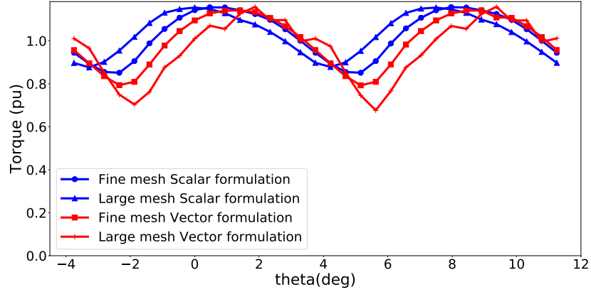
Figure 13: Torque
