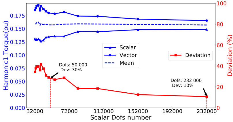
Figure 15: Torque: Harmonic 1
