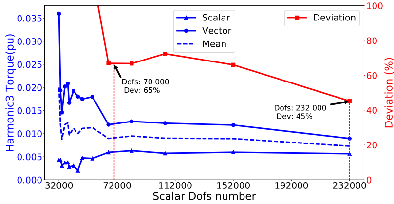
Figure 16: Torque: Harmonic 3
