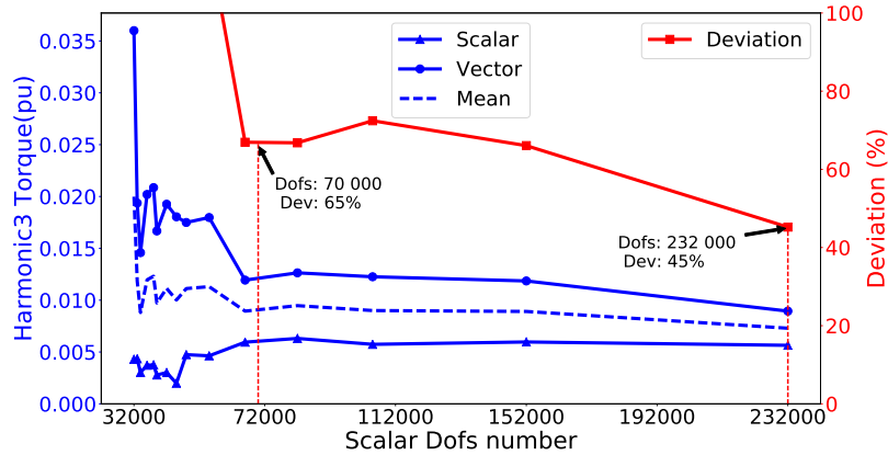
Figure 16: Torque: Harmonic 3
