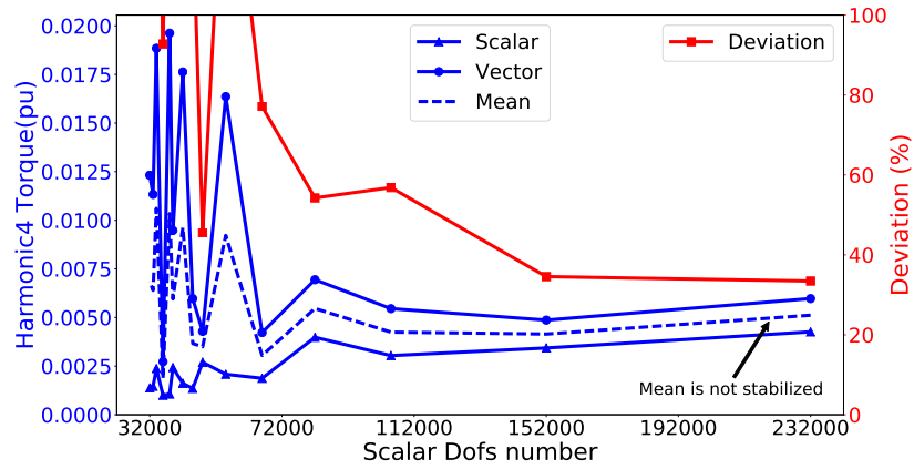
Figure 18: Torque: Harmonic 4
