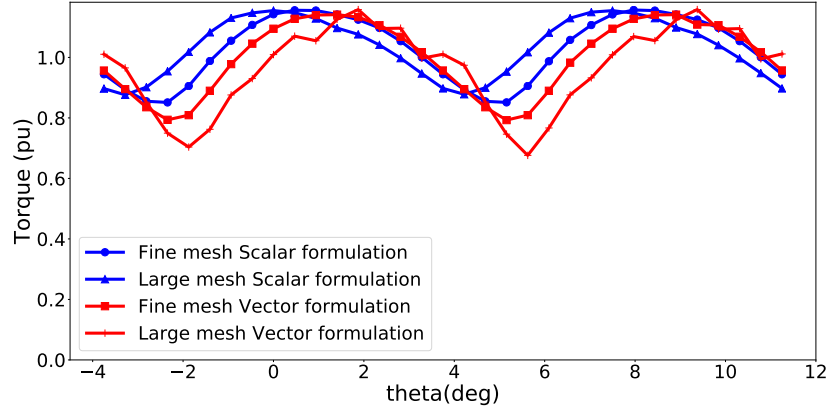
Figure 13: Torque
