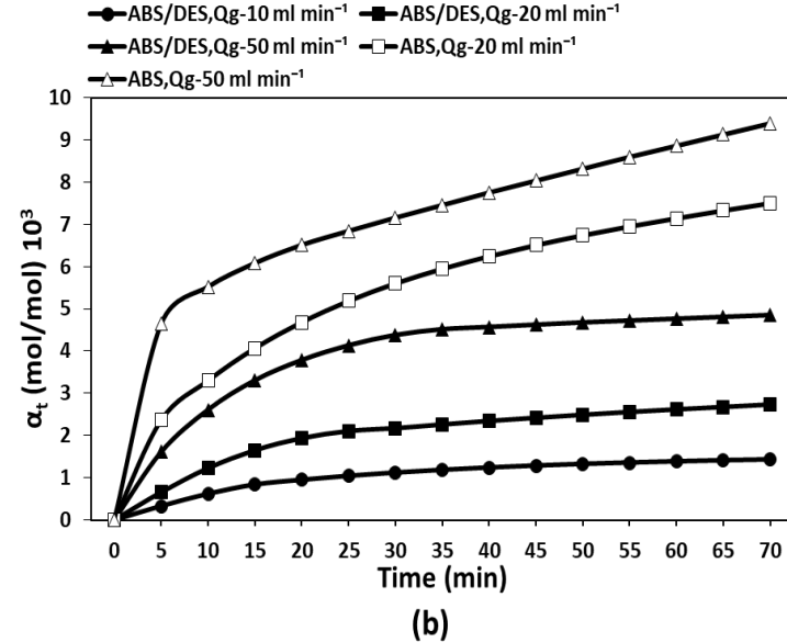
Figure 4 CO 2 loading \alpha_t of the IL (a) [emim] [MS] and (b) [emim] [DCA] during coupled absorption/desorption (ABS/DES) and single module absorption (ABS) against operation time
