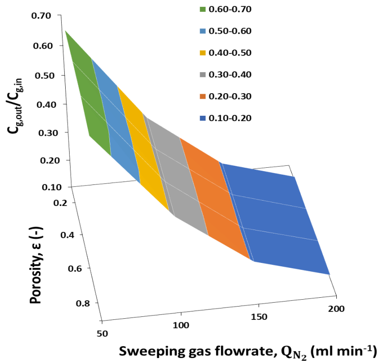
Figure 10 Effect of sweeping gas flowrate and porosity on the outlet concentration of CO 2 in the feed stream for IL [emim][MS]
