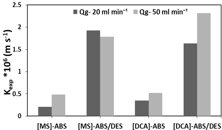
Figure 7 Experimental mass transfer coefficient, K_{exp} , for \text{CO}_2 absorption in ILs [emim] [MS] ([MS]) and [emim] [DCA] ([DCA]) during coupled absorption/desorption (ABS/DES) and single module absorption (ABS) at pseudo steady state
