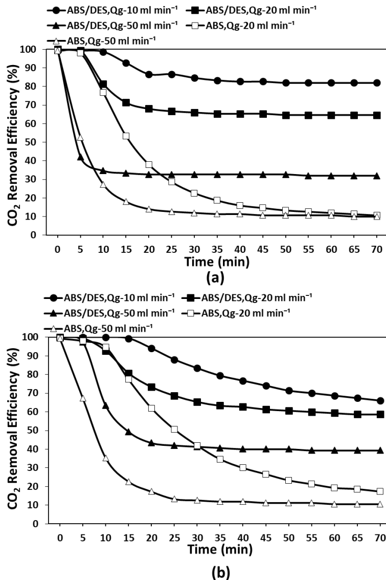
Figure 3 CO 2 removal efficiency of the membrane absorber for coupled absorption/desorption (ABS/DES) and single module absorption (ABS) against operation time for IL (a) [emim] [MS] and (b) [emim] [DCA]
