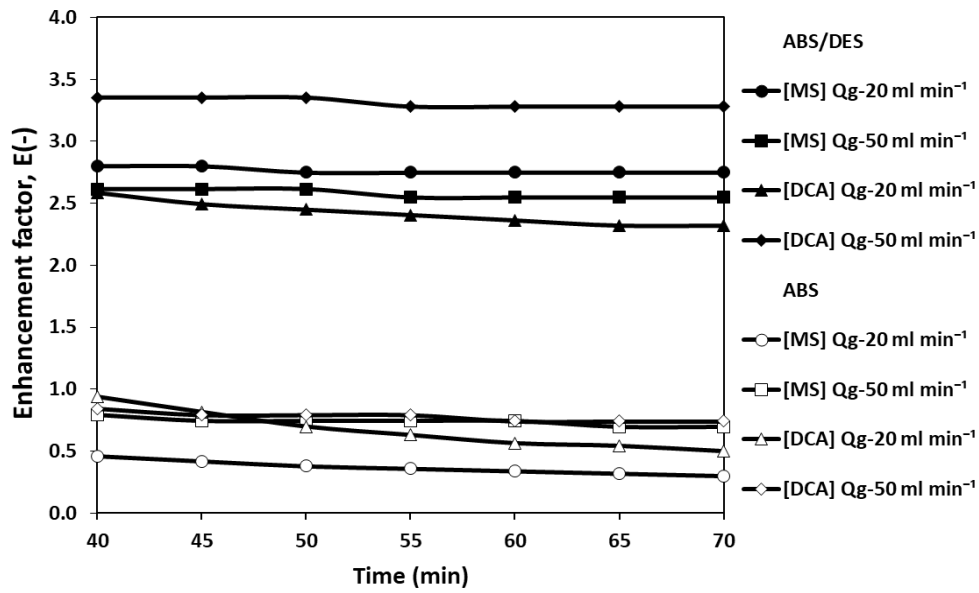
Figure 8 Enhancement factor, E, for CO 2 absorption in ILs [emim] [MS] ([MS]) and [emim] [DCA] ([DCA]) during coupled absorption/desorption (ABS/DES) and single module absorption (ABS) at pseudo steady state
