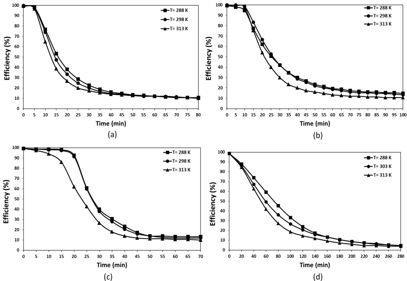
Figure 4. CO 2 removal efficiency against operation time for IL (a) [emim] [MeSO 4 ] ( Q_g = 20 \text{ ml min}^{-1} ), (b) [emim] [DCA] ( Q_g = 20 \text{ ml min}^{-1} ), (c) [emim] [EtSO 4 ] ( Q_g = 50 \text{ ml min}^{-1} ) and (d) [emim] [Ac] ( Q_g = 100 \text{ ml min}^{-1} ) at Q_{IL} = 60 \text{ ml min}^{-1} .
