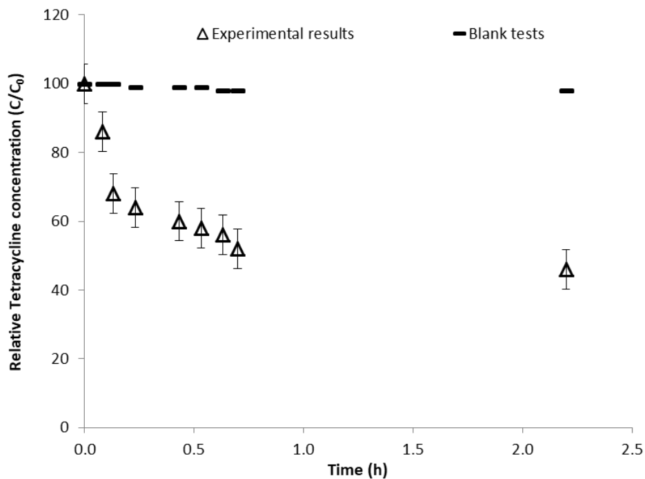
Figure 2: Evolution of % TC concentration (concentration/initial concentration).
