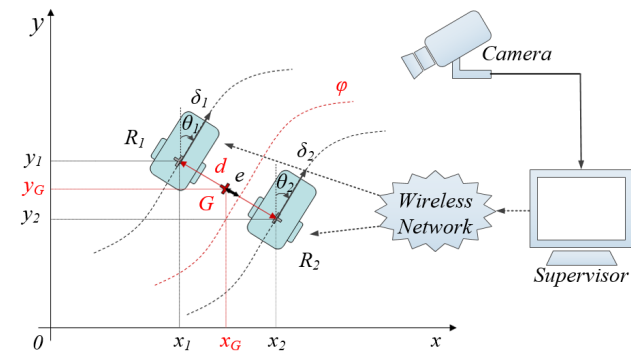
FIGURE 2. Setup of the cooperative robots platform.
