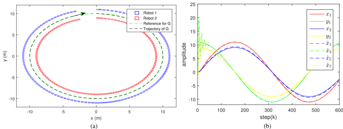
FIGURE 4. Trajectory of two cooperative robots (a) and the estimating performance of the estimator realized by the shift operator with \beta = 6 (b).
