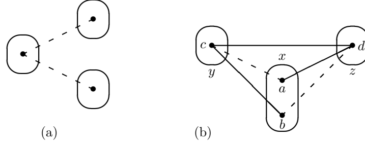
■ Figure 8 (a) The pattern V^- and (b) the associated broken-triangle pattern (BTP).
