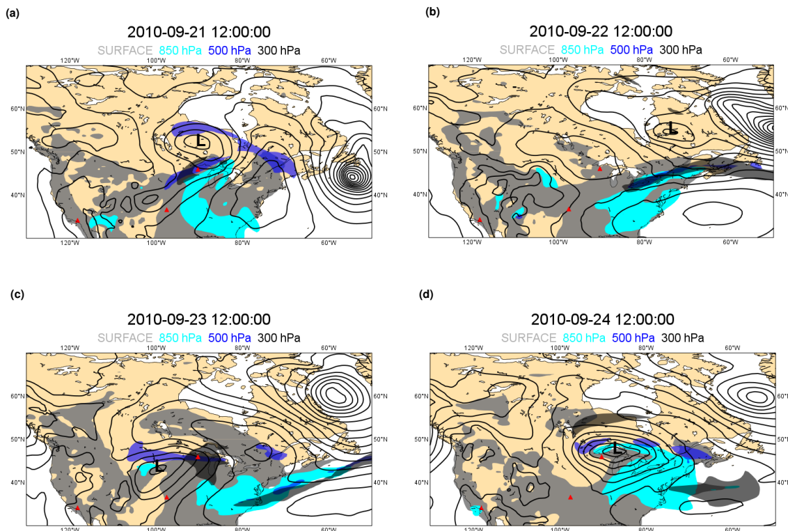
Figure 9. Transport of atmospheric CO 2 anomalies associated with the passage of low pressure systems over North America. The colours depict the CO 2 anomalies anomalies above the well-mixed background CO 2 at different vertical levels: grey near the surface, cyan at 850 hPa, blue at 500 hPa and dark grey at 300 hPa. The anomalies are defined as CO 2 dry molar fraction above the background value of 392 ppm for both near the surface and at the 850 hPa level; and above the background value of 388 ppm for the 500 and 300 hPa levels. The location of the TCCON sites are depicted by a red triangle. The black contours of mean sea level pressure show the location of the centre of the low pressure systems (L).
