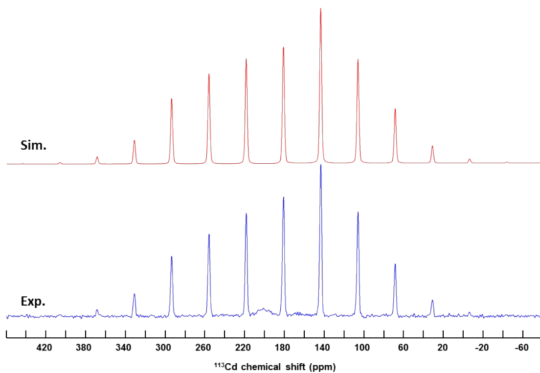
Figure S6. ^1\text{H} - ^{113}\text{Cd} CP-MAS (2.5 kHz) NMR spectrum of (\text{TDMP})\text{CdCl}_4 and its simulation by a single line at 181 ppm. The chemical shift anisotropy is 157 ppm and the asymmetry parameter is 0.79. The weak and broad line at \sim 200 ppm is attributed to a low amount of cadmium chloride impurity.
