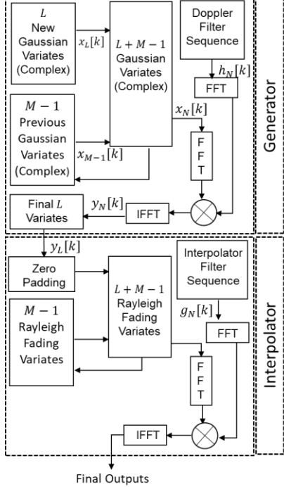
Figure 1: Block diagram of OLS-based channel emulator
