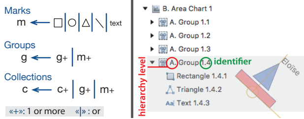
Fig. 3. StructGraphics visualization elements: marks, groups, and collections. Left: Their grammar. Right: An example of a visualization tree. We highlight a group that contains a rectangle, a triangle, and a text field.
