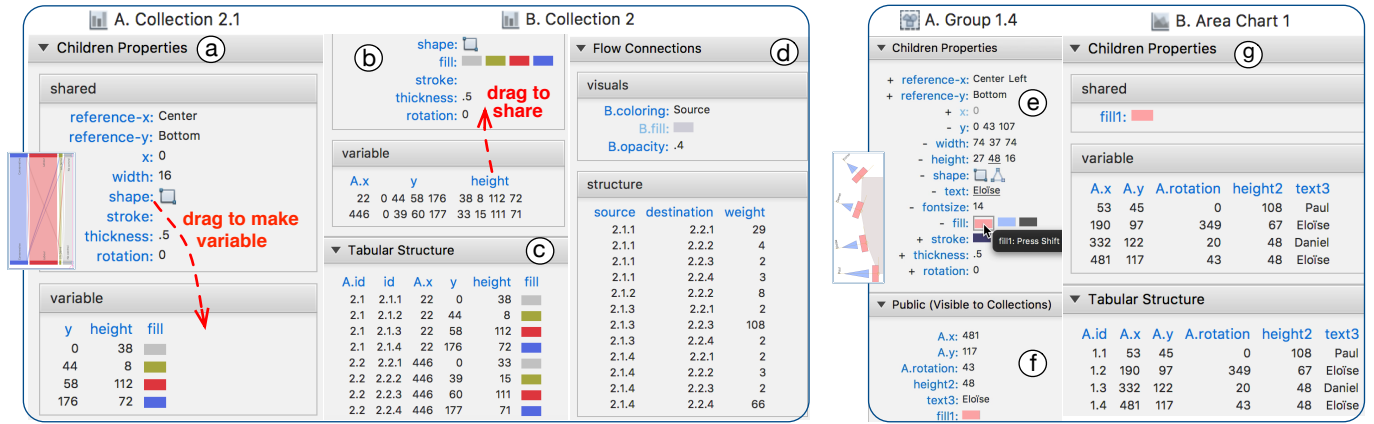
Fig. 5. Property structures of the visualizations in Fig. 1, as represented in the StructGraphics inspector. Left: (a) The children properties of the first A-level collection divided into two groups: shared and variable. (b) Part of the children properties of the B-level collection. (c) A tabular structure that summarizes all variable properties. (d) Structure of connections between nodes. Right: (e) Structure of the children properties of an A-level group. The user can choose which properties to make public. (f) Those properties are highlighted and appear in the “Public (Visible to Collections)” section. (g) The structure of children properties in the B-level collection. Observe that only public group properties are shown.
