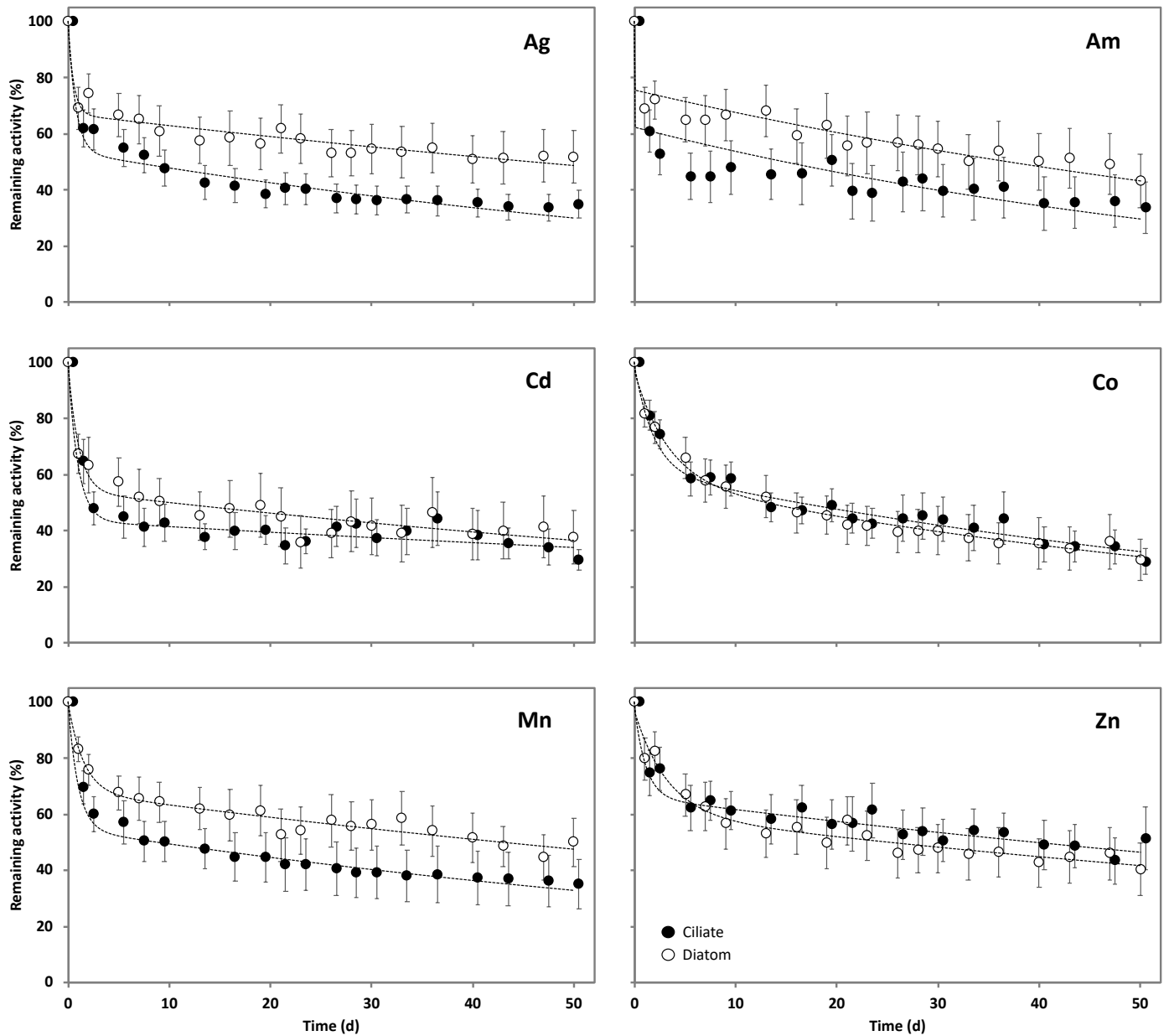
Figure 1. Whole-body depuration kinetics of dietary Ag, Am, Cd, Co, Mn, and Zn in Pacific cupped oysters Crassostrea gigas (n=10, % remaining activities, mean \pm SE) fed ciliate Uronema marinum and phytoplankton Thalassiosira pseudonana . Parameters and statistics of the depuration kinetics are given in Table 2.
