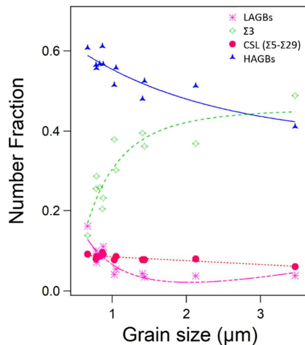
Fig. 6 – Evolution with grain size of the fraction of the different types of grain boundaries in UFG sintered Ni.
