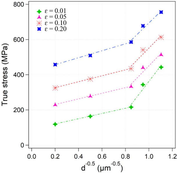
Fig. 13 – Effect of grain size on stress at different deformation levels.
