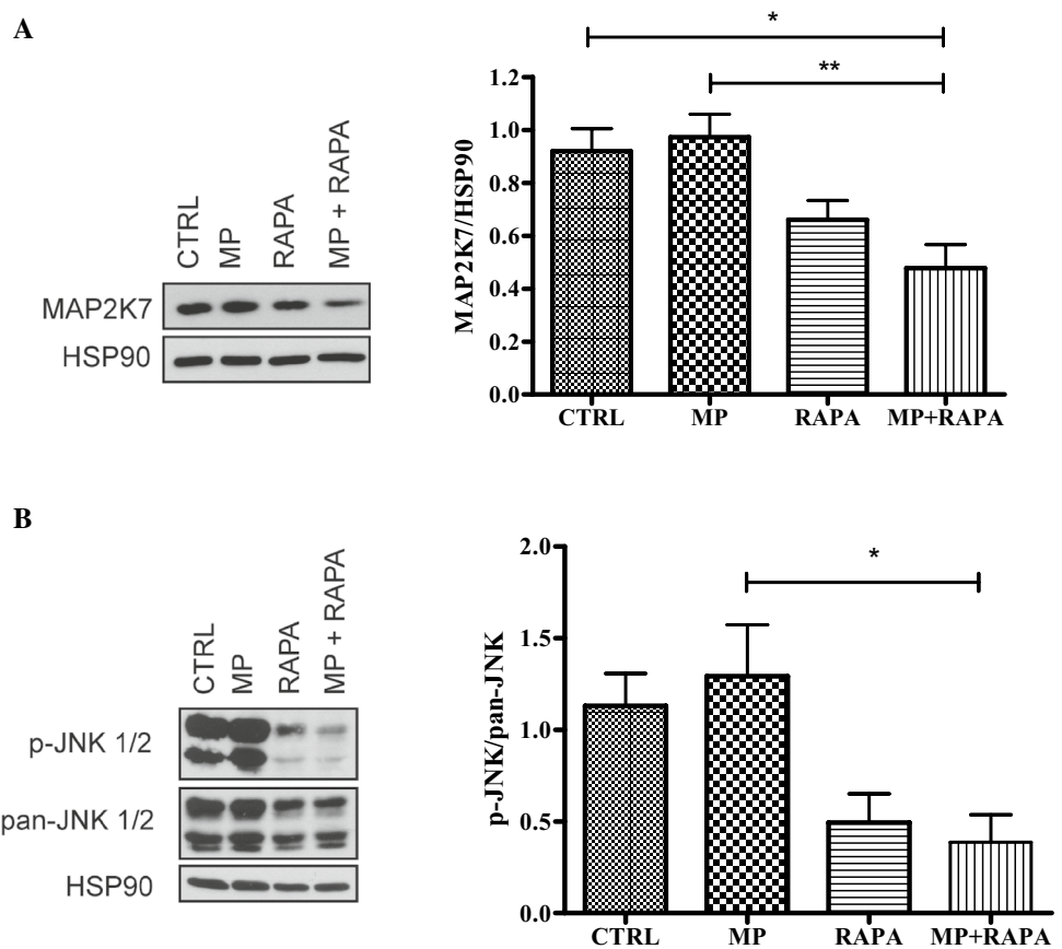
Fig. 5 a Protein expression of MAP2K7 by western blot analysis on CCRF-CEM cells untreated (CTRL) treated with MP (50 \mu M), RAPA (1 nM) and MP+RAPA for 72 h. MAP2K7 expression evaluated in cells treated and untreated for 72 h normalized by HSP90 protein; one-way ANOVA analyses: p=0.0022 , Bonferroni's post-test *p value <0.05 ; **p value <0.01 . The data are reported as means \pm SE of three independent experiments performed in triplicate. b Protein expression of p-JNK and pan-JNK by western blot analysis on CCRF-CEM cells untreated (CTRL) treated with MP (50 \mu M), RAPA (1 nM) and MP+RAPA for 72 h. P-JNK expression evaluated in cells treated and untreated for 72 h in respect to pan-JNK protein. One-way ANOVA analyses: p=0.0022 , Bonferroni's post-test *p value <0.05 ; **p value <0.01 . The data are reported as means \pm SE of three independent experiments performed in triplicate.
