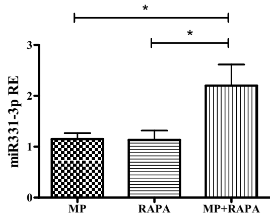
Fig. 4 Relative expression (RE) of miR-331-3p after treatment with MP (50 \mu M), RAPA (1 nM) and MP+RAPA for 72 h. One-way ANOVA ( p = 0.023 ) and Bonferroni post-test *p value < 0.05 . The data are reported as means \pm SE of three independent experiments performed in triplicate
