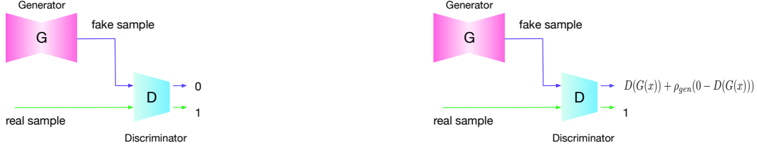
FIGURE 1. Comparison of GAN with and without generator impact. On left : vanilla GAN, on right : proposed GAN with weighted labels.
