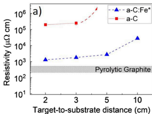
Fig. 5. a) Resistivity measurements of a-C and a-C:Fe* thin films deposited on Si by DCMS at different target-to-substrate distances. Resistivity value for pyrolytic graphite (from [46] is also displayed using logarithmic scale. The dashed lines are only to guide the eye. b) SEM micrograph of the film topography for an a-C:Fe sample deposited at 10 cm.
